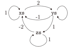
Figure 3: An example clique of streams to illustrate well-definedness.
